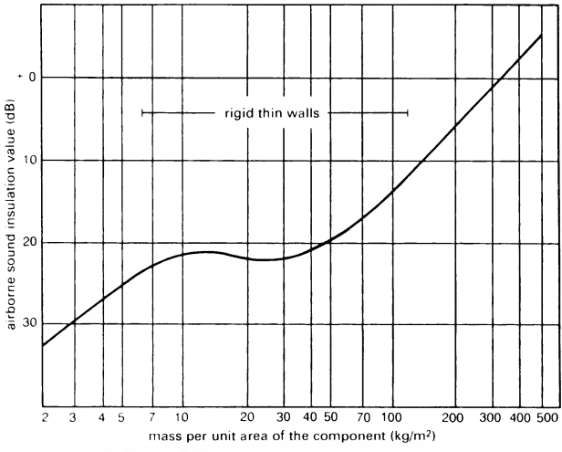
⑤ Airborne sound insulation, weight/unit surface area and component thickness (Gäsele)
